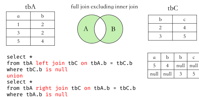
图 4.12: full join excluding inner join
