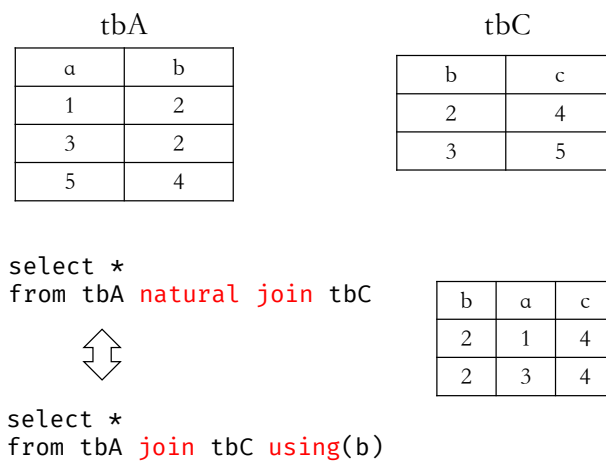
图 4.14: natural join
