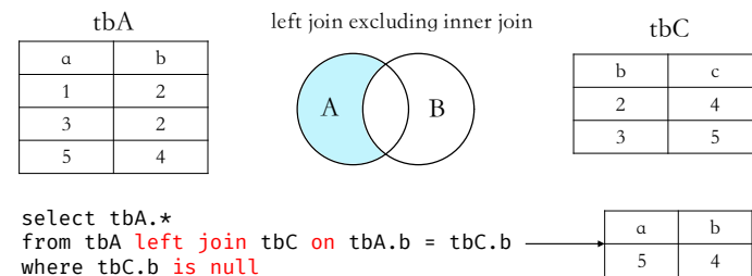
图 4.11: left join excluding inner join
