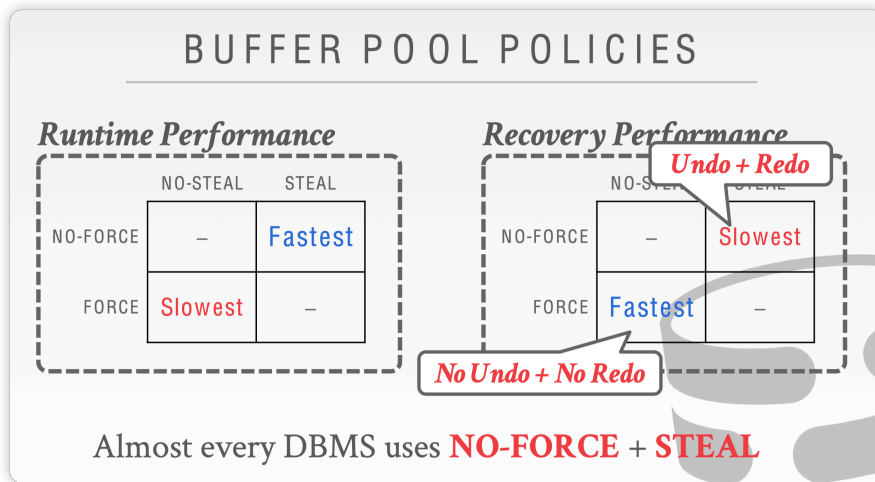
图 10.10: Buffer Pool Policies
