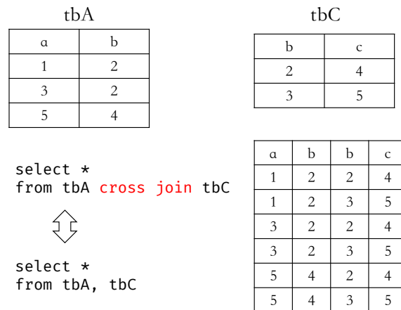
图 4.13: cross join
